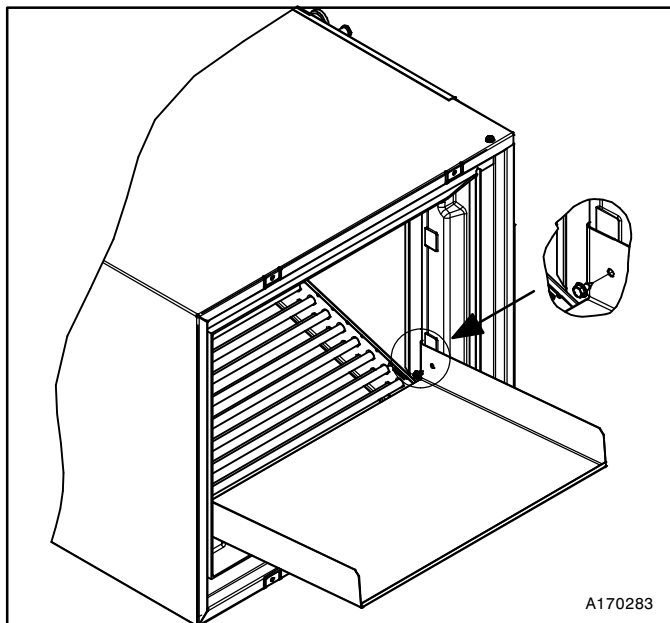
Figure 6 – Condensate Pan Extension Cork Tape Location
