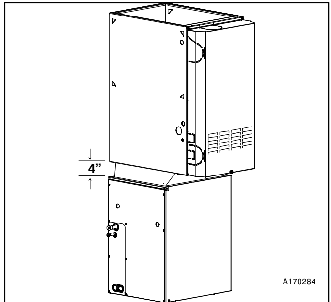
Figure 3 – Downflow Installation with Coil Rotated 90°
