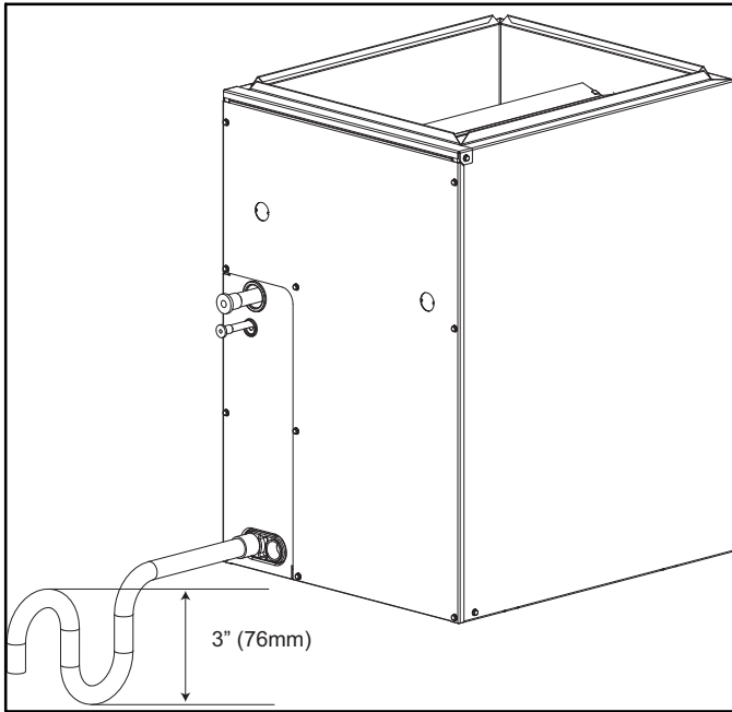
Figure 10 – Condensate Trap
